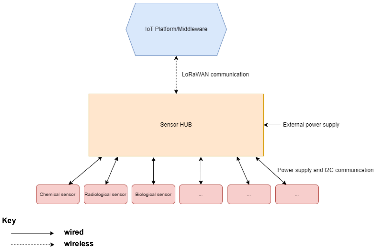
Figure 1 — Schematic overview of the HUB and the communication units
