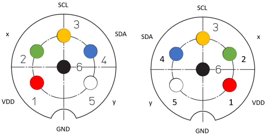
HUB (Case) and sensor with male connector
